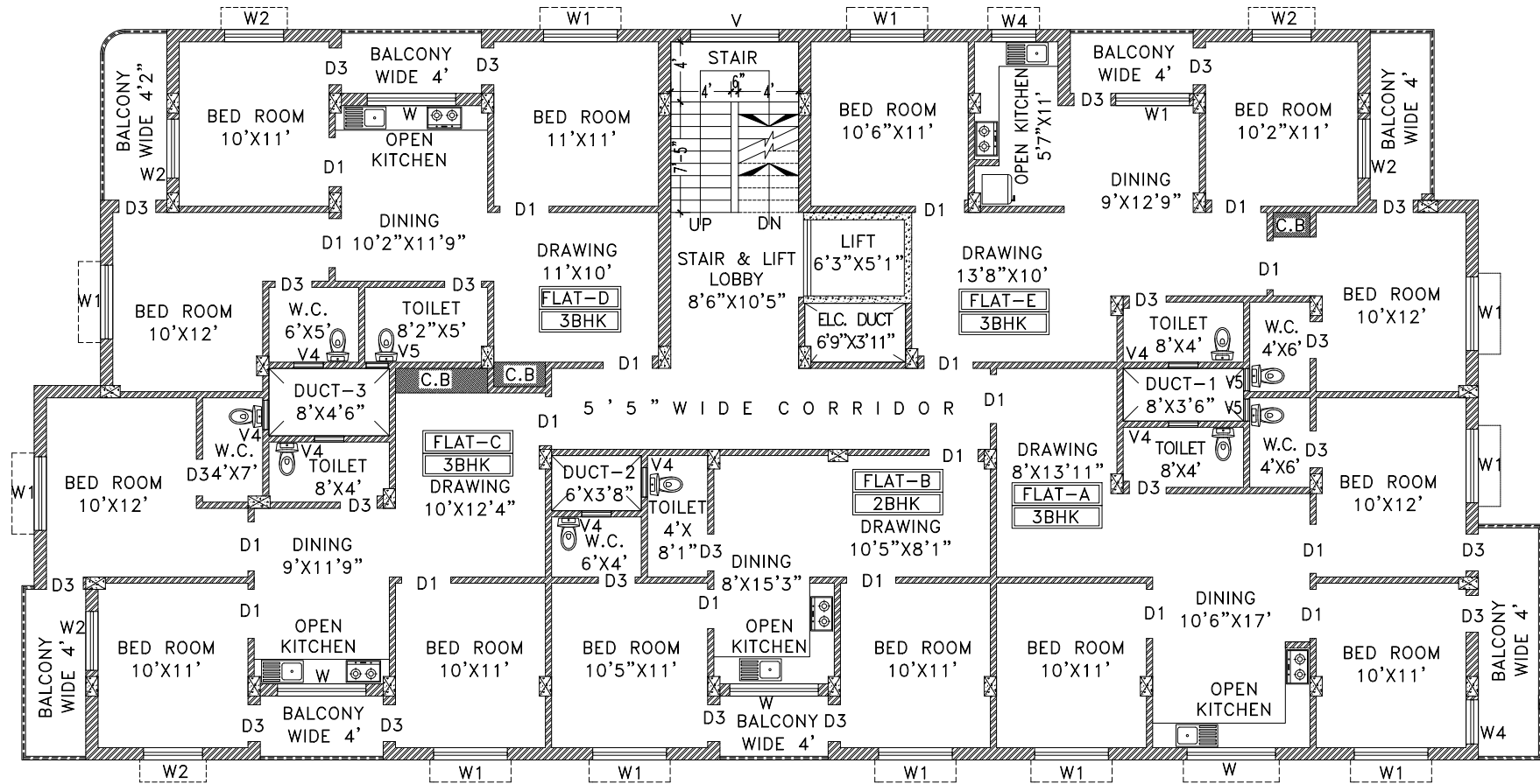
(B) TYPICAL FLOOR PLAN SCALE: 1:100
